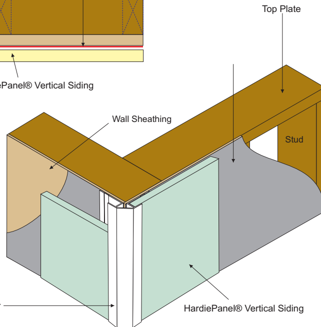
Xtreme Trim™ Blunt Panel Outside Corner
